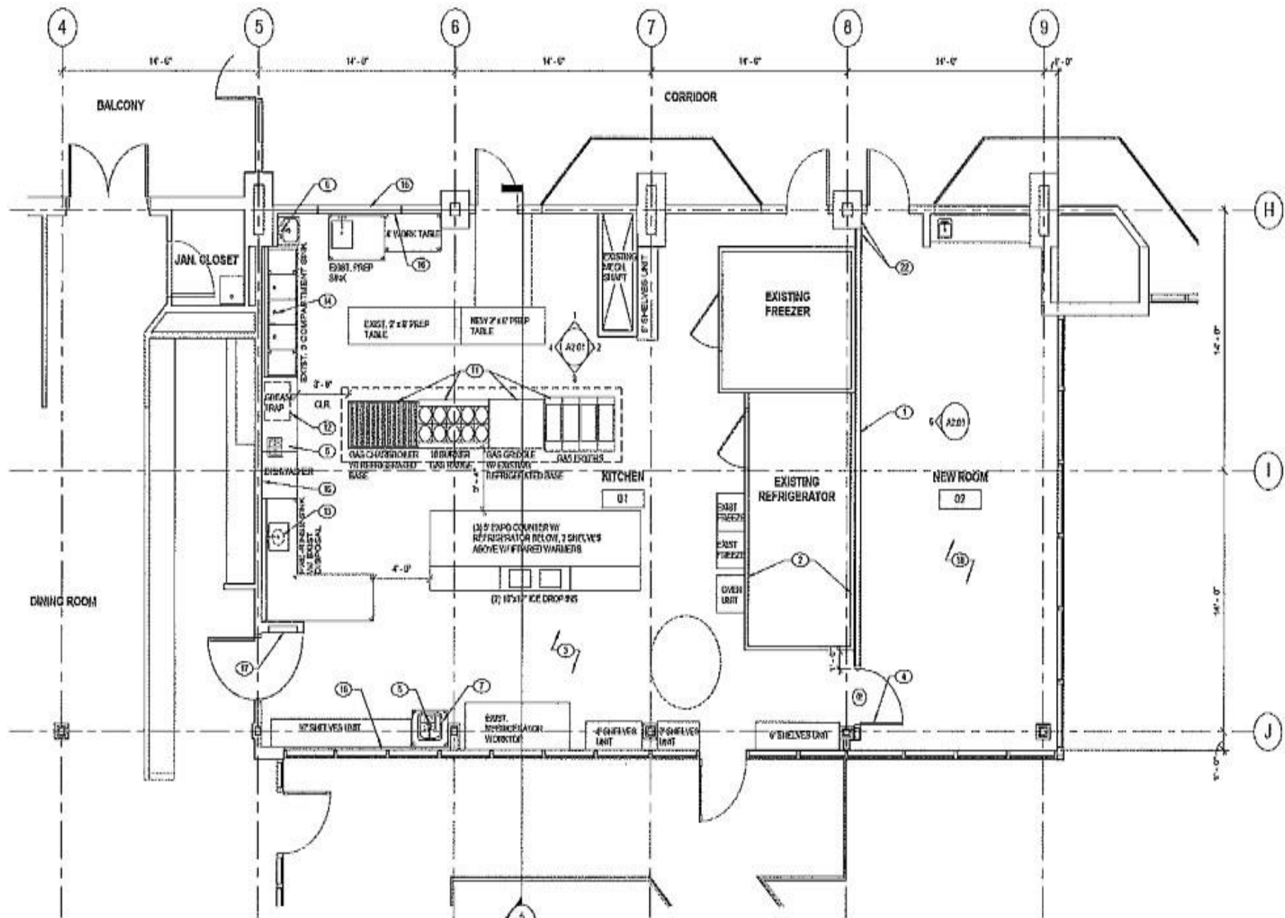
A FLOOR PLAN - UPPER LEVEL SCALE: 1/4" = 1'-0"
